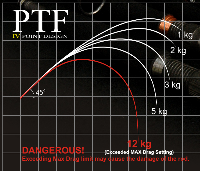
Taka-Si / Ji 5814 Max.Drag 10kg Simulation PTF Curve
